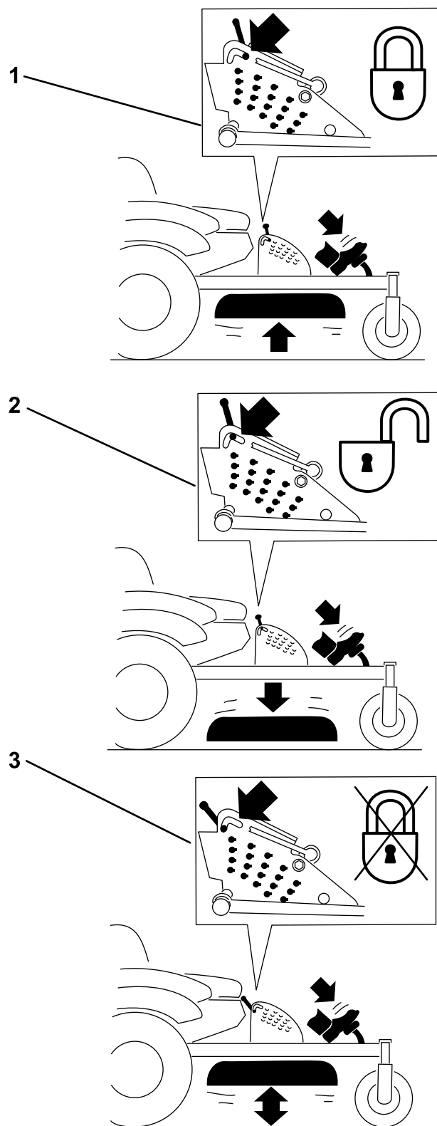
Figur 26 Transportlåsepositioner
