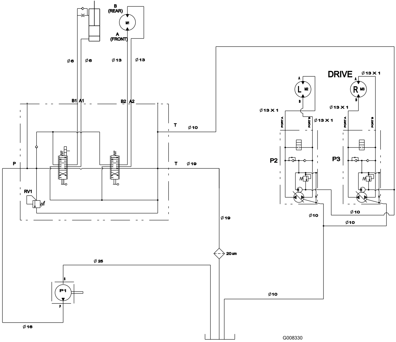
Hydraulik - Modell 22970 (Rev. A)
