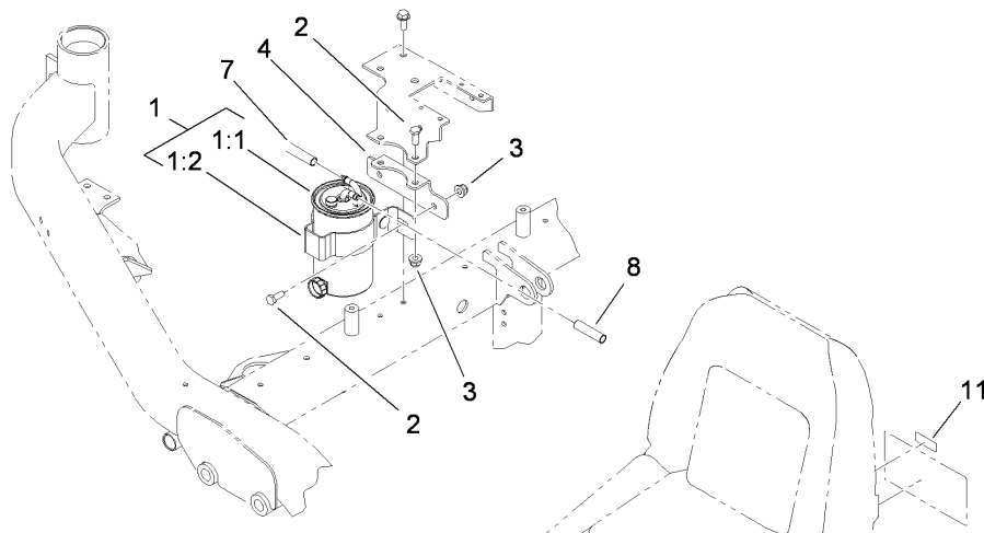
FILTER INSTALLATION
