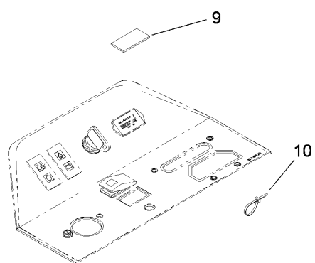
PLUG INSTALLATION
