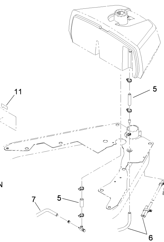
FUEL HOSE INSTALLATION
