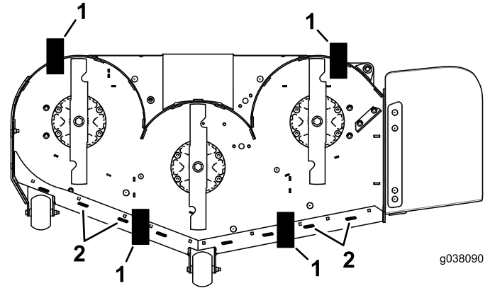
Figure 90 Bottom view
