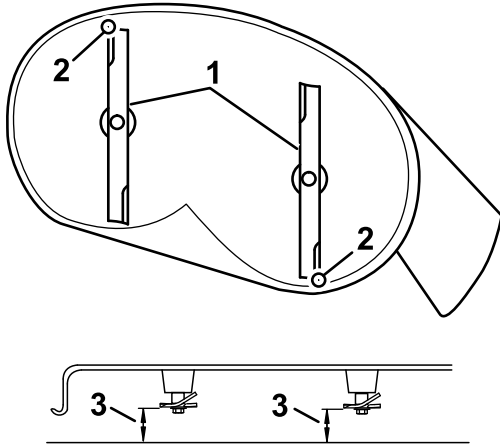
Figure 66 Mower Decks with 2 Blades
