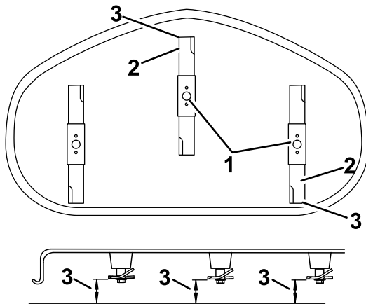
Figure 67 Mower Decks with 3 Blades
