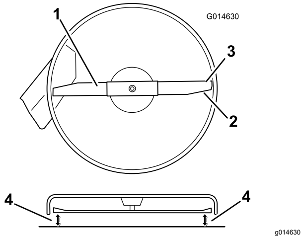
Figure 57 Mower Decks with 1 Blade
