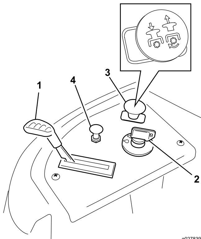
Figure 5 Control Panel
